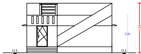
FRONT ELEVATION
