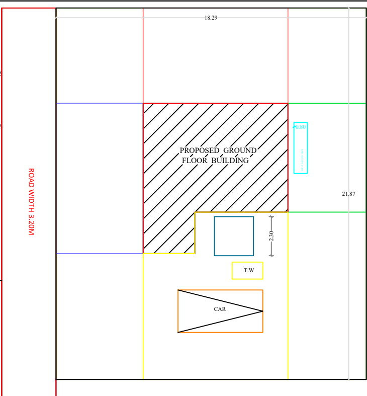
KEY PLAN
