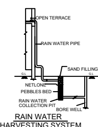
RAIN WATER HARVESTING SYSTEM
