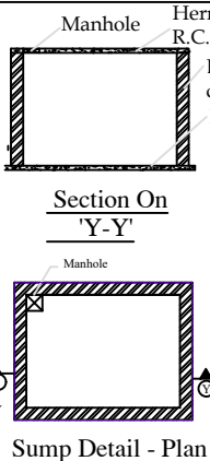
Sump Detail - Plan
