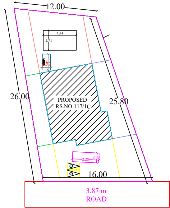
SITE PLAN
