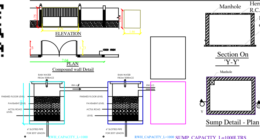
SECTION OF RAIN WATER PERCOLATION BED
