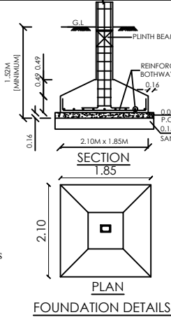
FOUNDATION DETAILS
