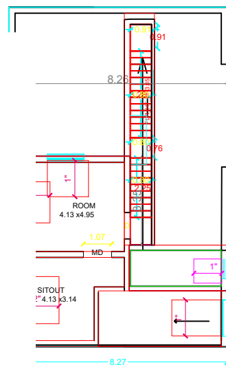
EXS-PRO. FIRST FLOOR PLAN
