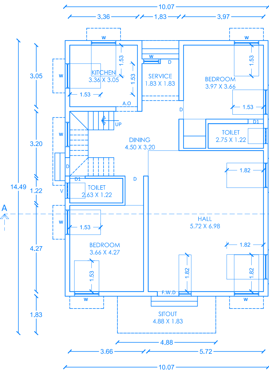
ND FLOOR PLAN
