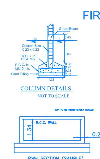
COLUMN DETAILS
