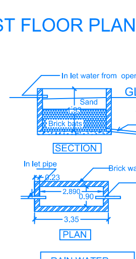
RAIN WATER HARVESTING TANK
