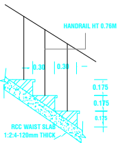
STAIR CASE STEPS SCALE 1:25
