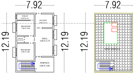
PRO.GROUND FLOOR PLAN
