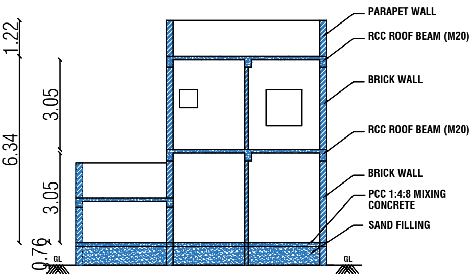
SECTION NO -"AB"
