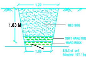
TRIAL PIT DETAILS NOT TO SCALE
