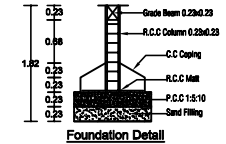
Foundation Detail
