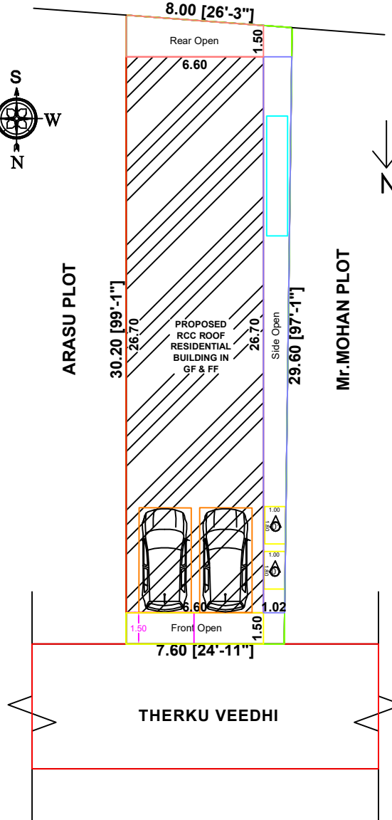
SITE PLAN [1:100]
