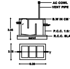
Septic tank detail
