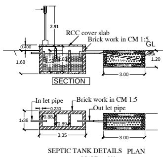
SEPTIC TANK DETAILS PLAN SCALE 1:200
