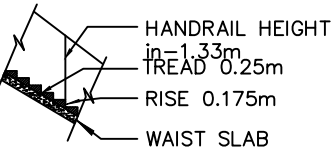
STAIRCASE DETAILS
