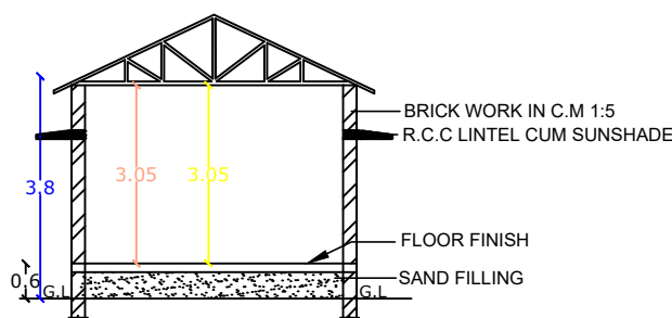
SECTION ON XX
