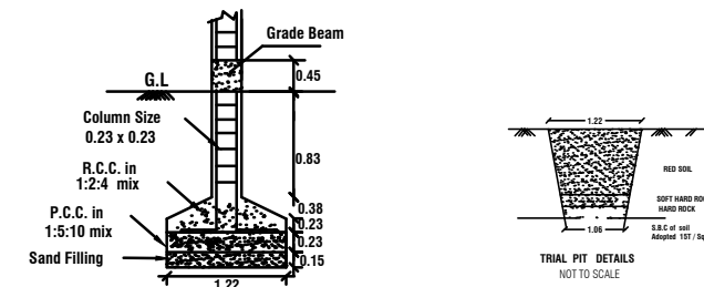
COLUMN DETAILS NOT TO SCALE
