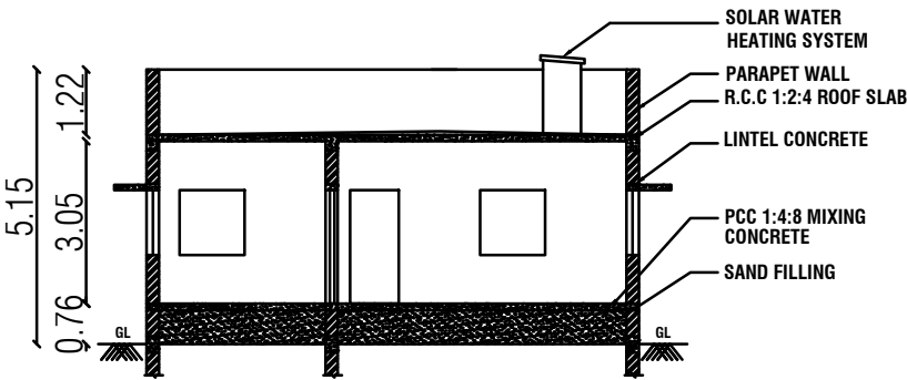
SECTION NO -"AB"
