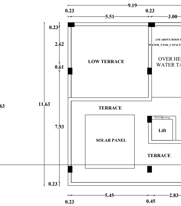
TERRACE FLOOR
