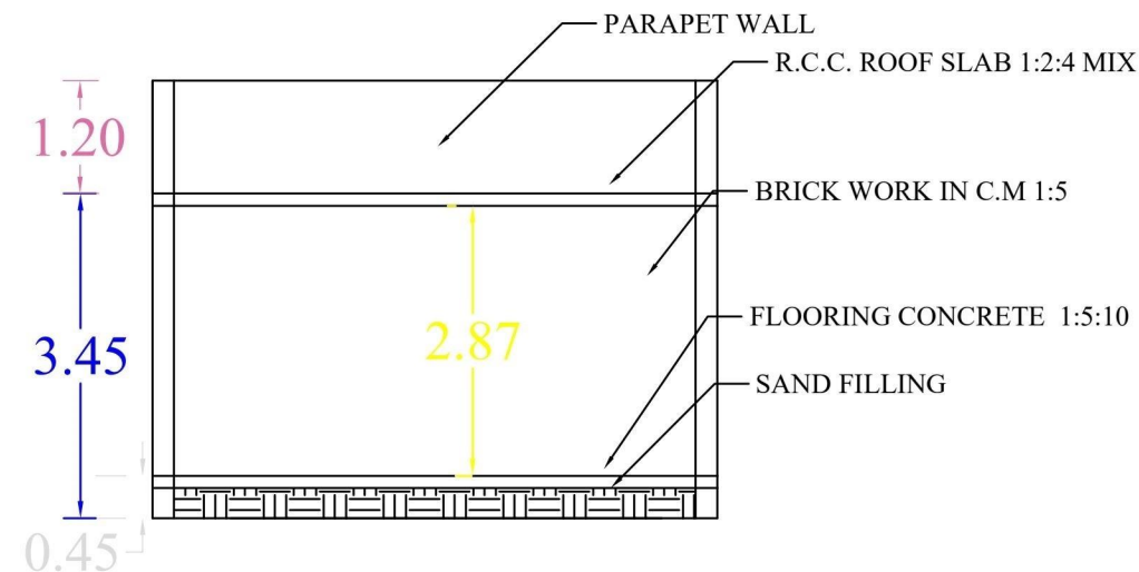
SECTION XX-XX
