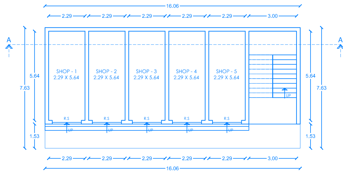
EXT.GROUND FLOOR PLAN
