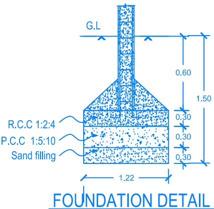
FOUNDATION DETAIL
