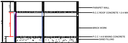
CROSS SECTION
