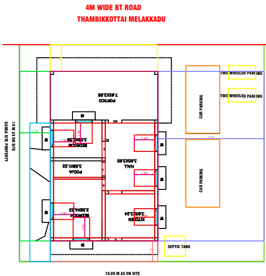
SITE PLAN
