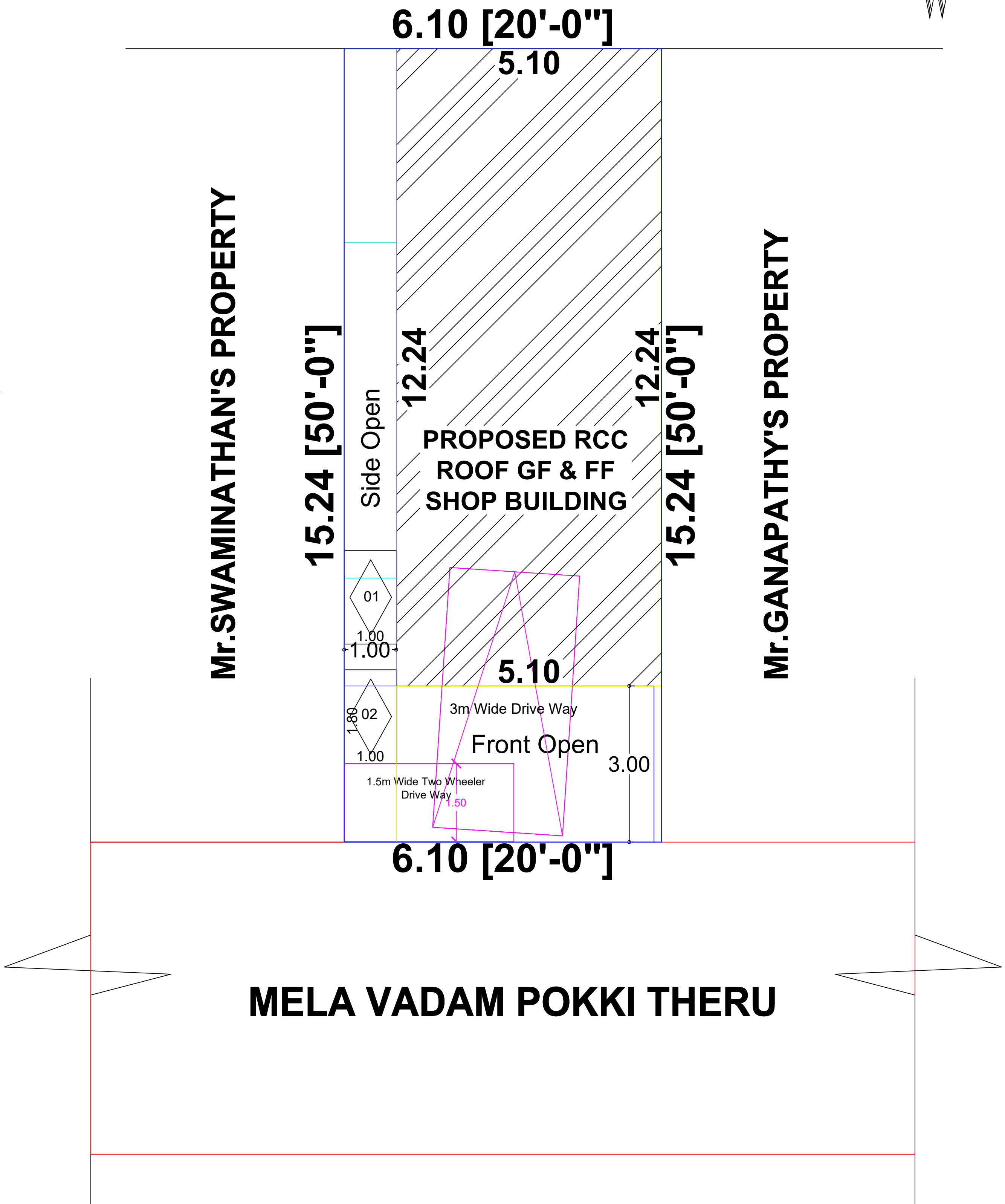
SITE PLAN [1:100]
