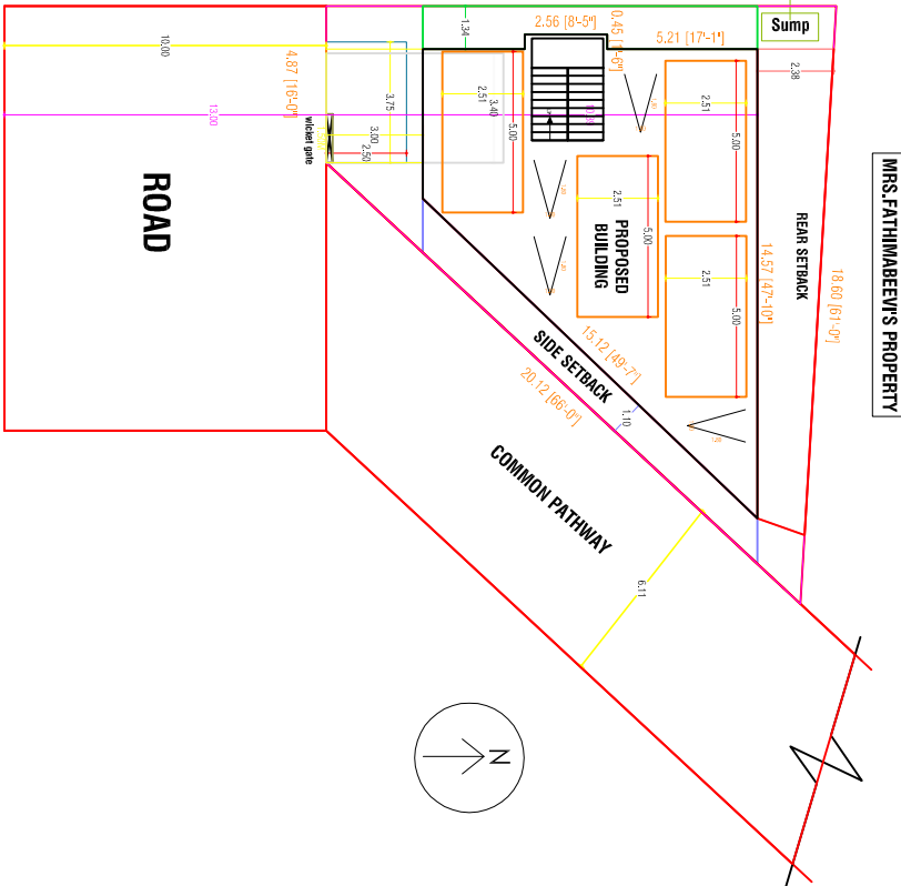
SITE PLAN [1:100]
