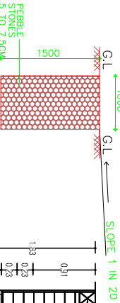
SECTION OF PEBBLE TRENCH
