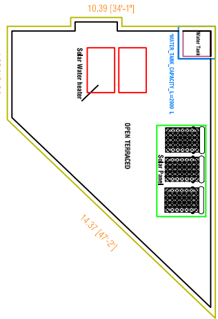
TERRACED FLOOR PLAN
