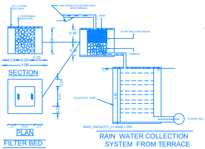
RAIN WATER COLLECTION SYSTEM FROM TERRACE
