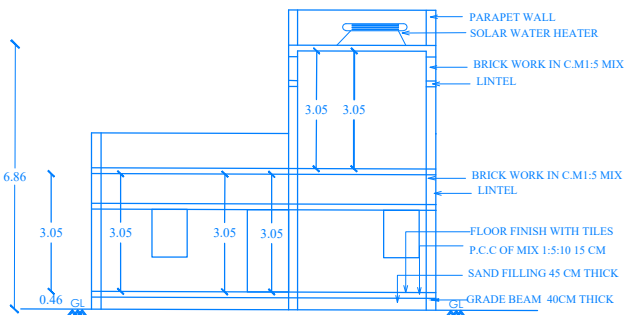
SECTION-AB
