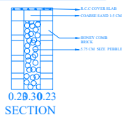
PERCOLATION PIT SECTION PLAN
