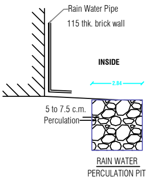
RAIN WATER PERCUSSION PIT
