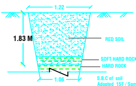
TRIAL PIT DETAILS NOT TO SCALE
