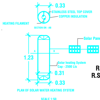
PLAN OF SOLAR WATER HEATING SYSTEM SCALE 1:50
