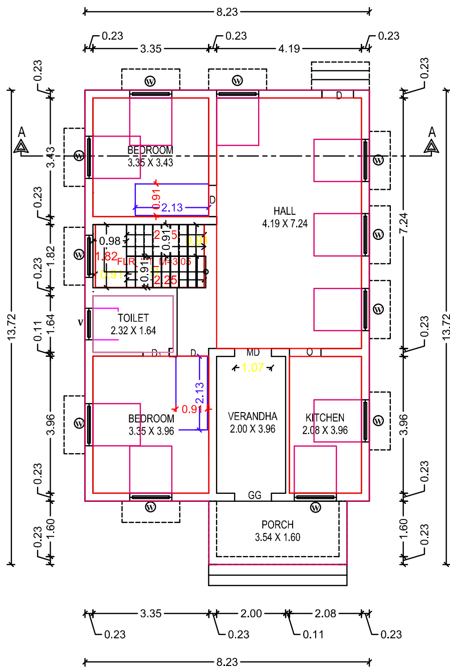
1d Floor Plan
