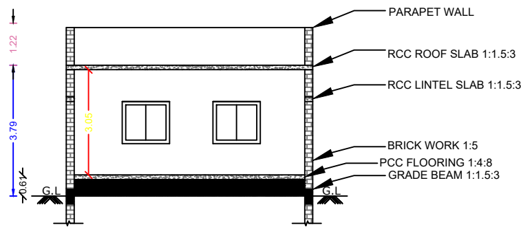
SECTION AT AB
