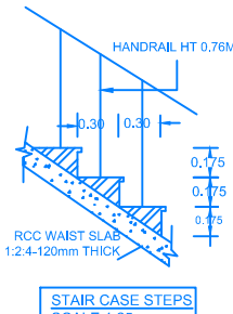
STAIR CASE STEPS SCALE 1:25
