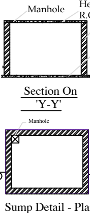
Sump Detail - Plan
