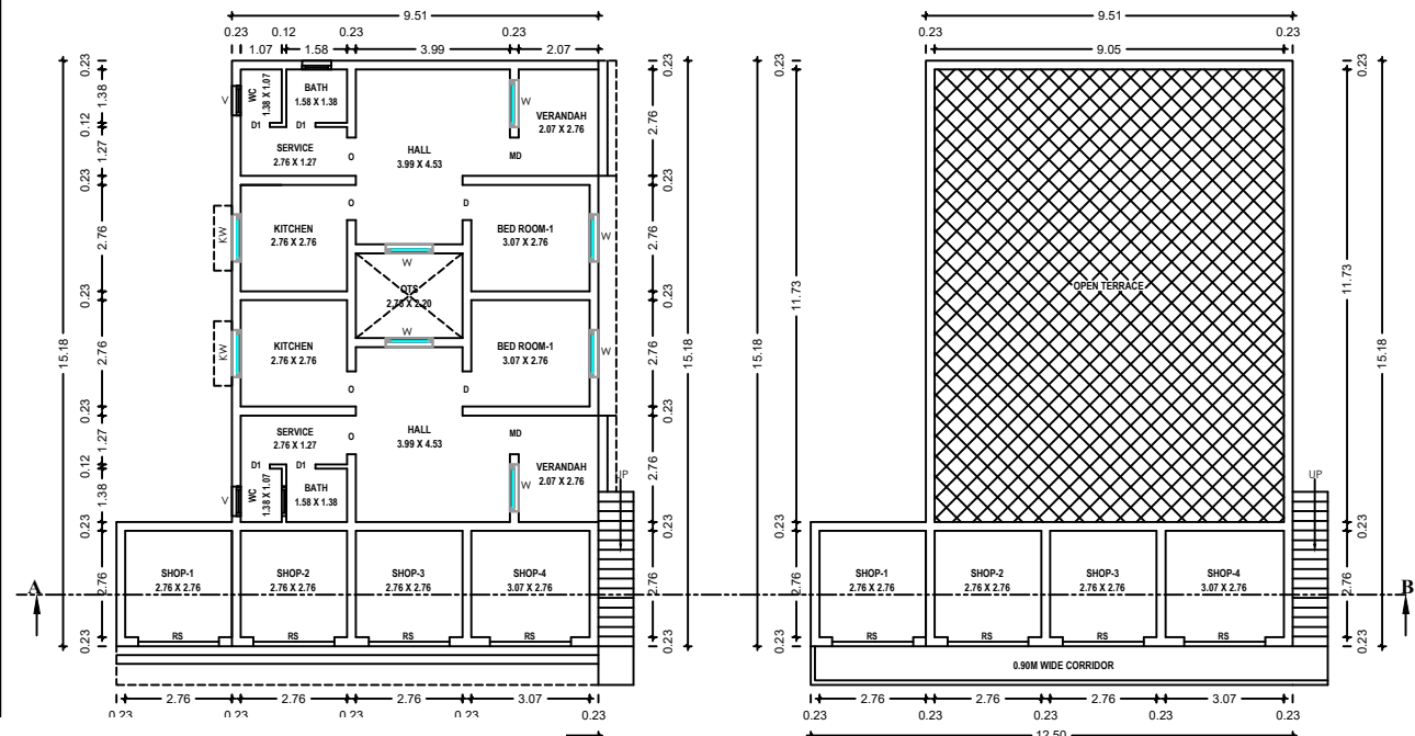
PRO.FIRST FLOOR PLAN
