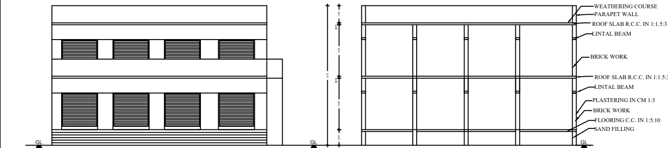
FRONT ELEVATION
