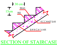
SECTION OF STAIRCASE
