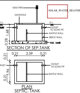
PLAN SEPTIC TANK
