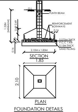
FOUNDATION DETAILS
