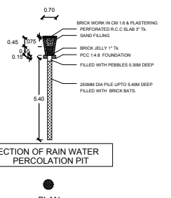
SECTION OF RAIN WATER PERCOLATION PIT
