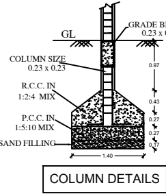
COLUMN DETAILS
