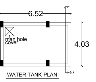
WATER TANK-PLAN
