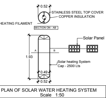
PLAN OF SOLAR WATER HEATING SYSTEM Scale: 1:50
