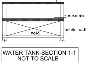
WATER TANK-SECTION 1-1 NOT TO SCALE
