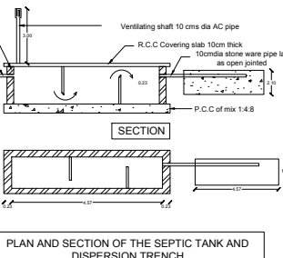
PLAN AND SECTION OF THE SEPTIC TANK AND DISPERSION TRENCH
