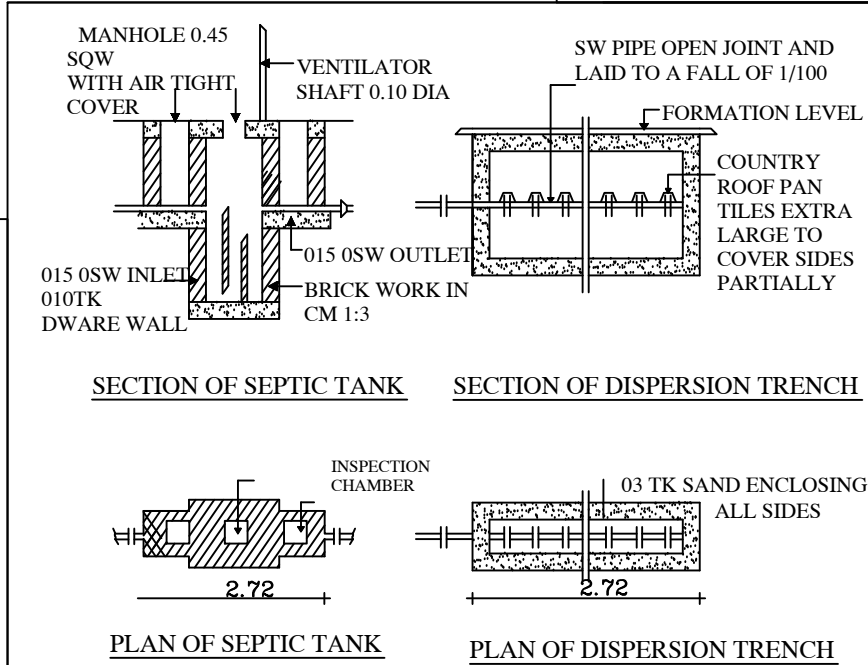
PLAN OF SEPTIC TANK
