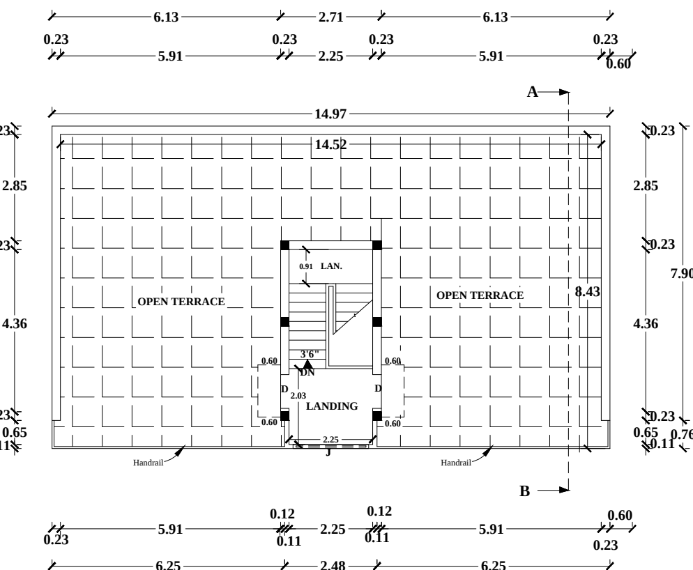
HEAD ROOM FLOOR PLAN
