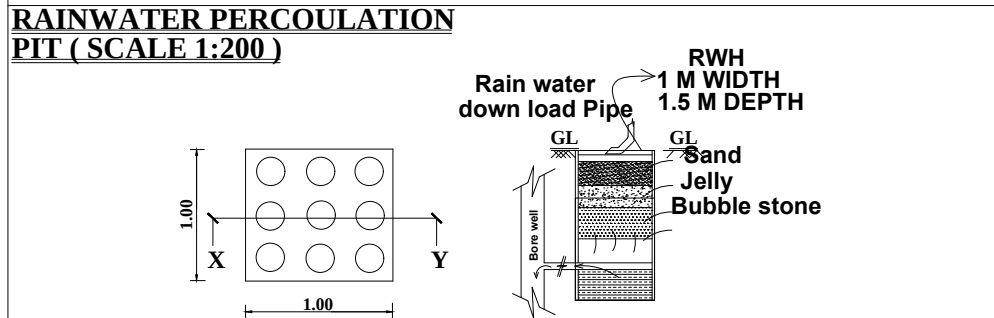
PLAN SECTION ON XY
