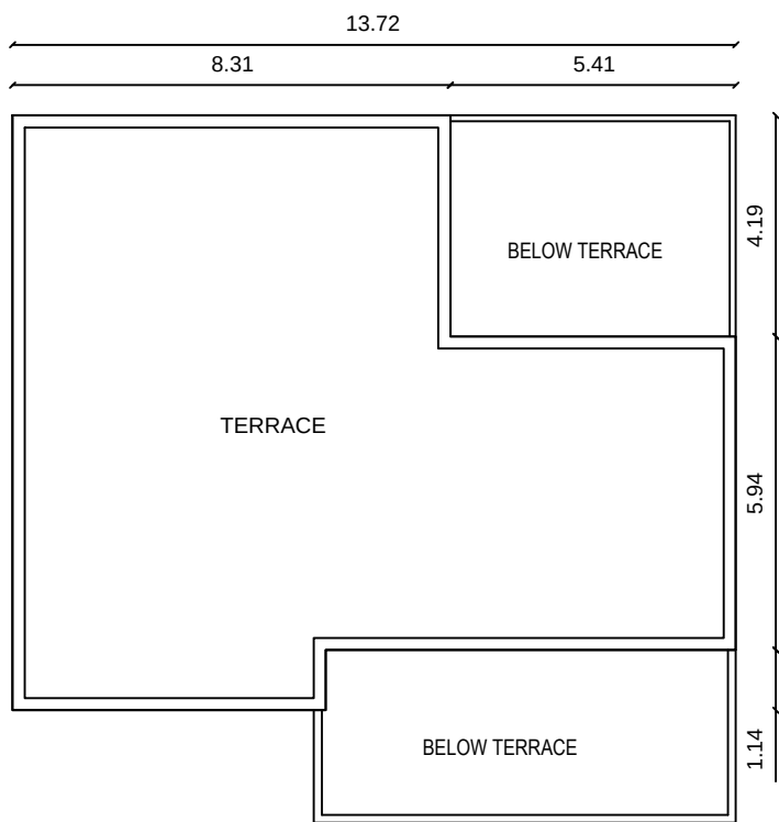
TERRACE PLAN
