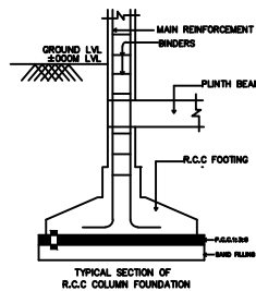
TYPICAL SECTION OF R.C.C. COLUMN FOUNDATION
