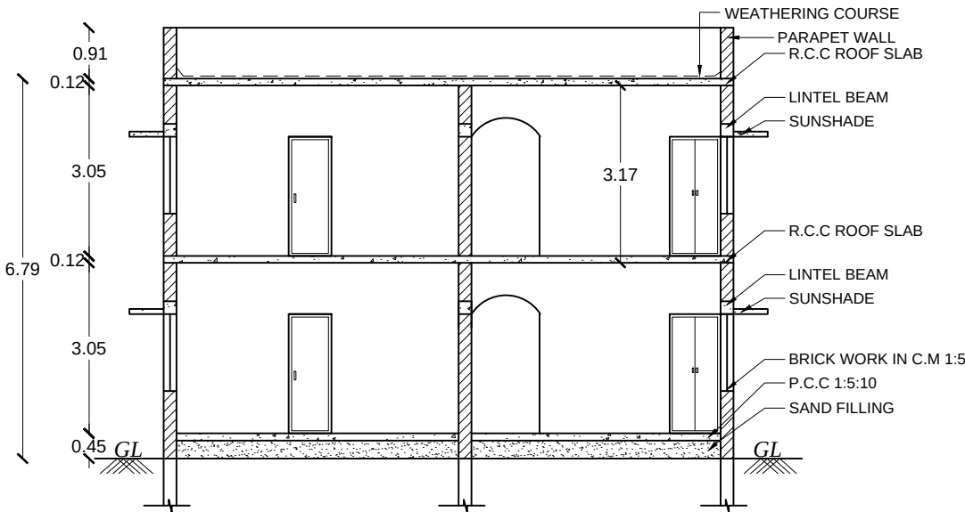
SECTION ON-X-Y
