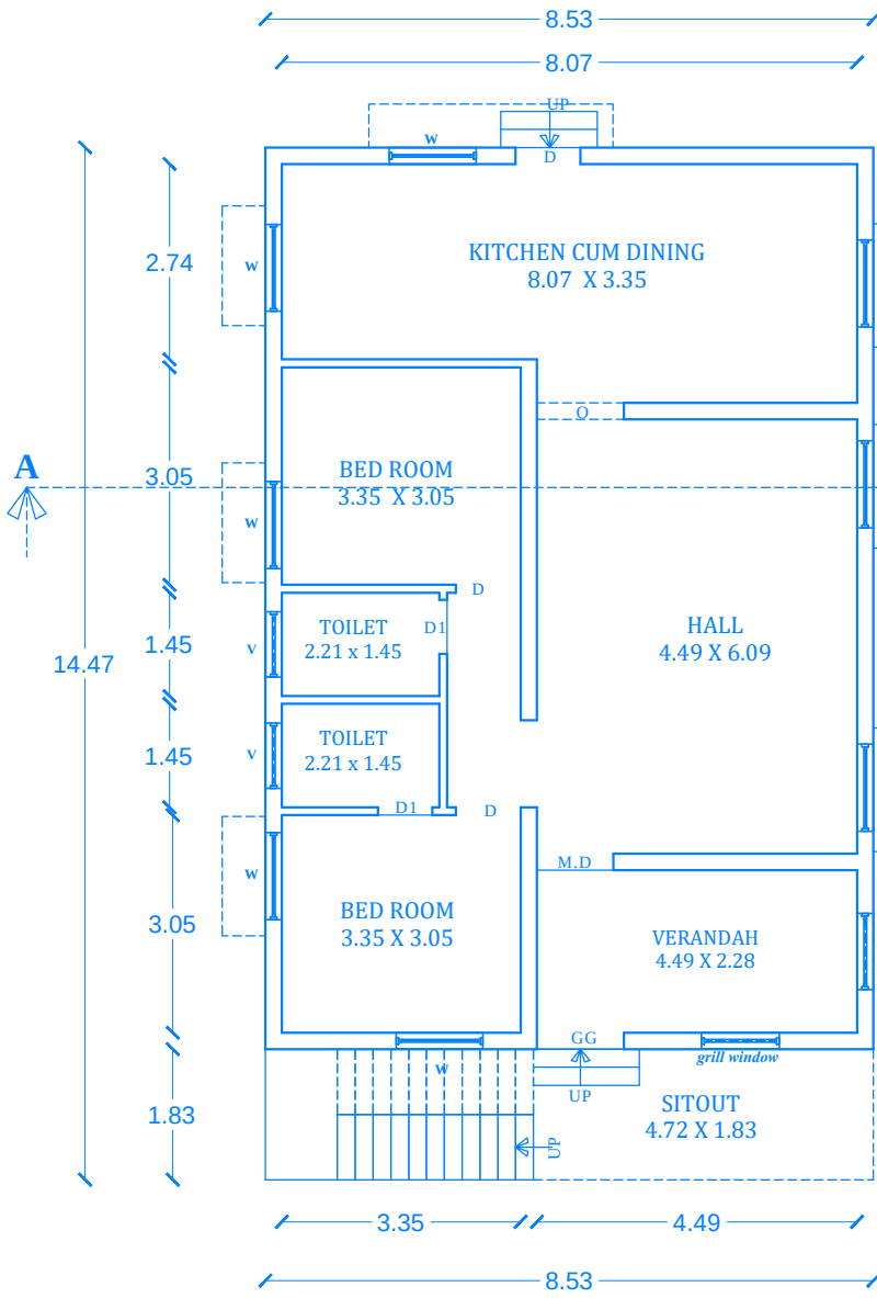
FLOOR PLAN
