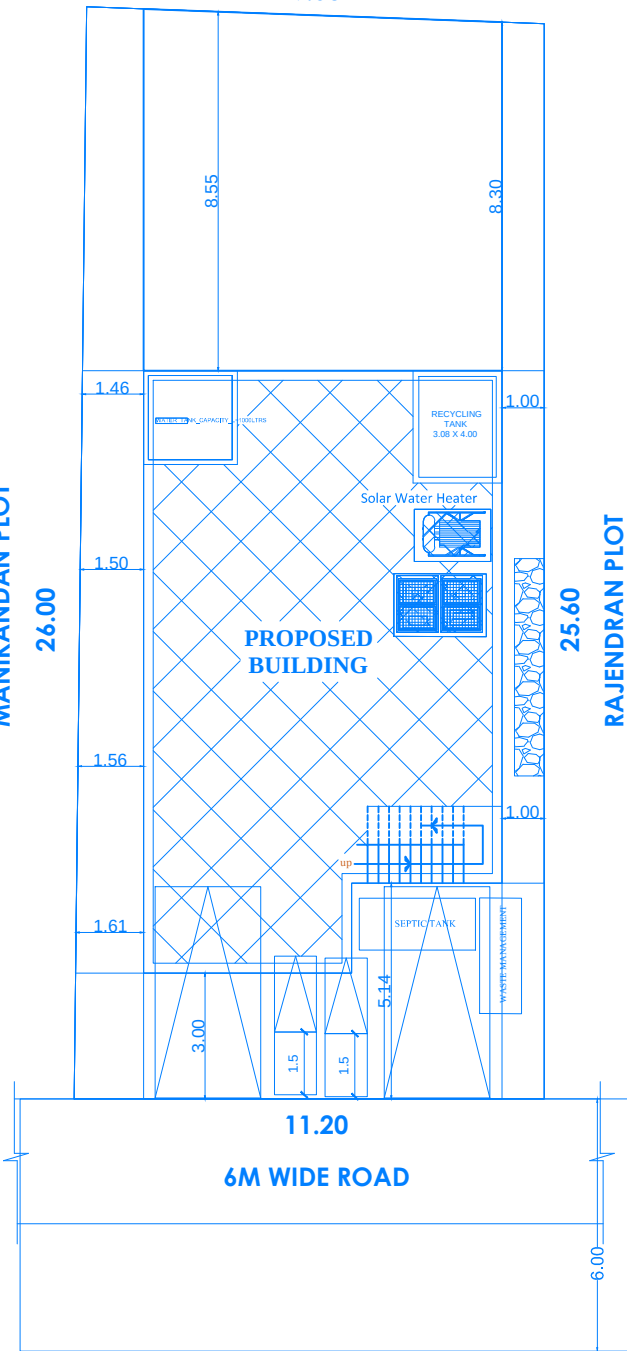
SITE PLAN
