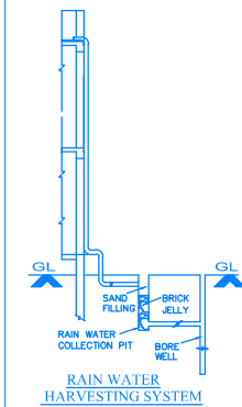
RAIN WATER HARVESTING SYSTEM
