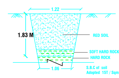
TRIAL PIT DETAILS NOT TO SCALE
