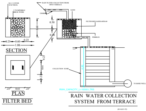
RAIN WATER HARVESTING PERCOLATION BED
