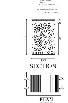
RAIN WATER HARVESTING PERCOLATION BED
