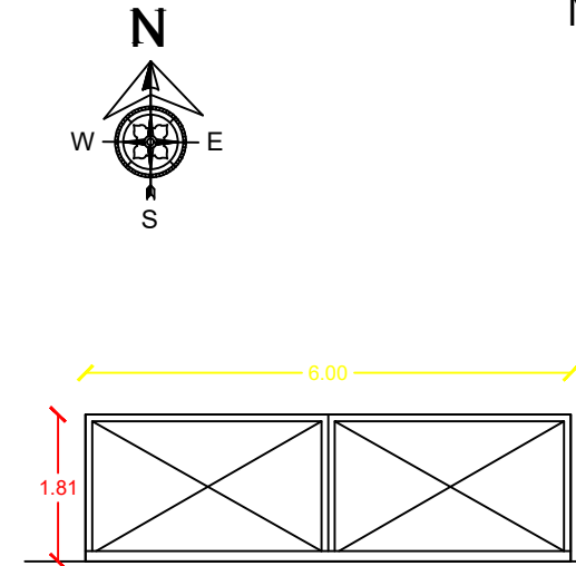
MAIN GATE
