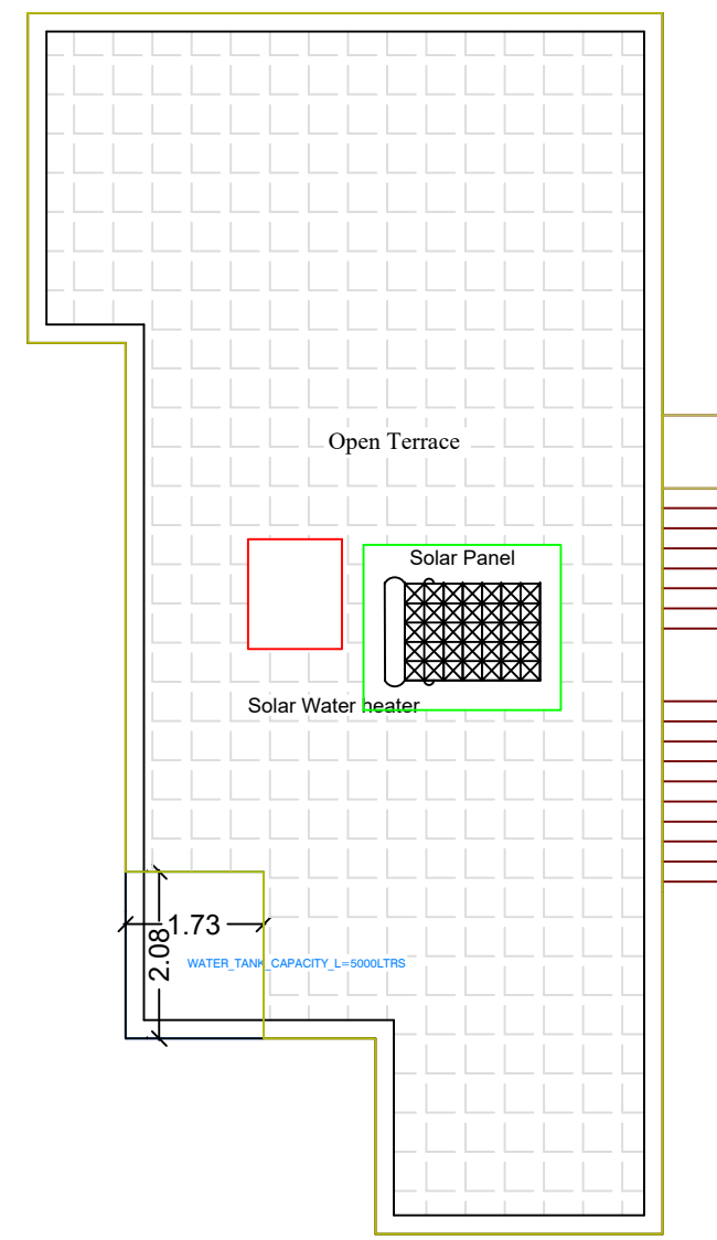
TERRCED FLOOR PLAN
