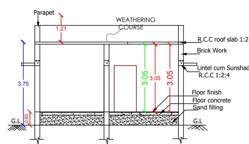
SECTION ON "A S"
