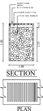
RAIN WATER HARVESTING PERCOLATION BED
