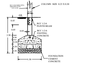
FOUNDATION DETAILS Scale 1:50
