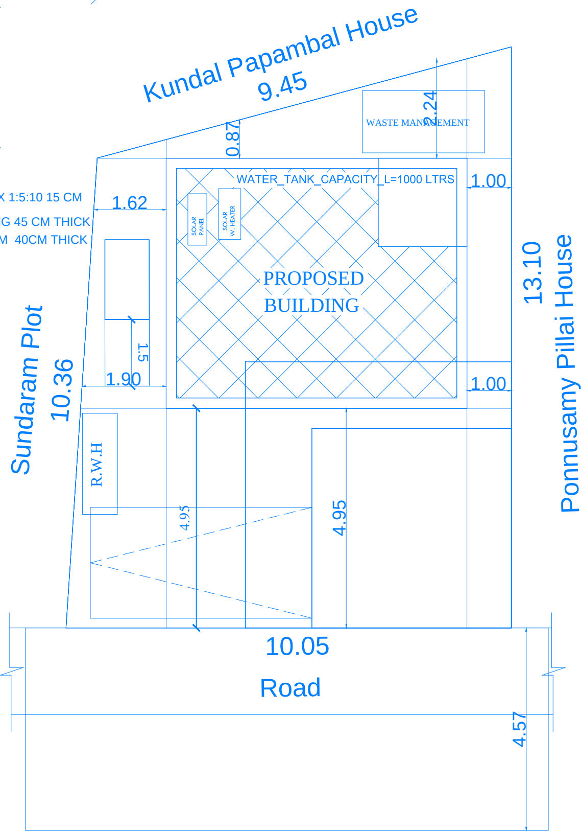
SITE PLAN
