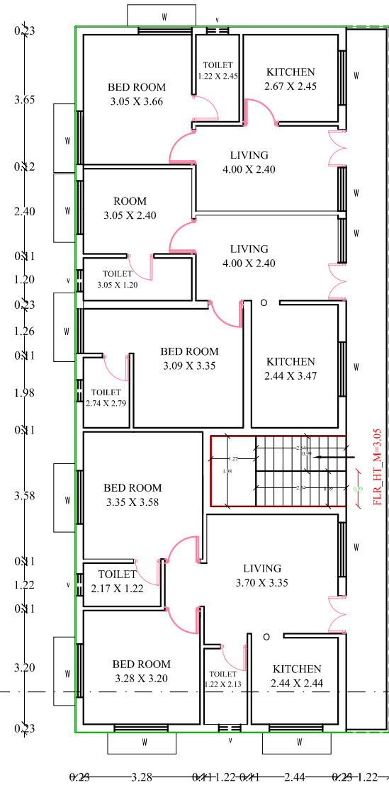
EXIST. FIRST FLOOR PLAN
