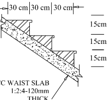
STAIR CASE STEPS SCALE 1:25
