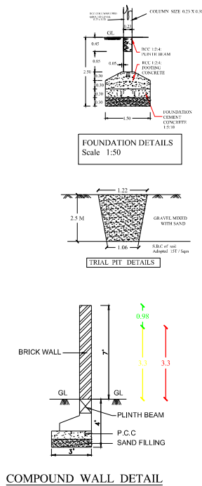
FOUNDATION DETAILS Scale: 1:50
