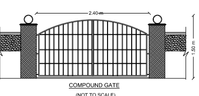
COMPOUND GATE (NOT TO SCALE)
