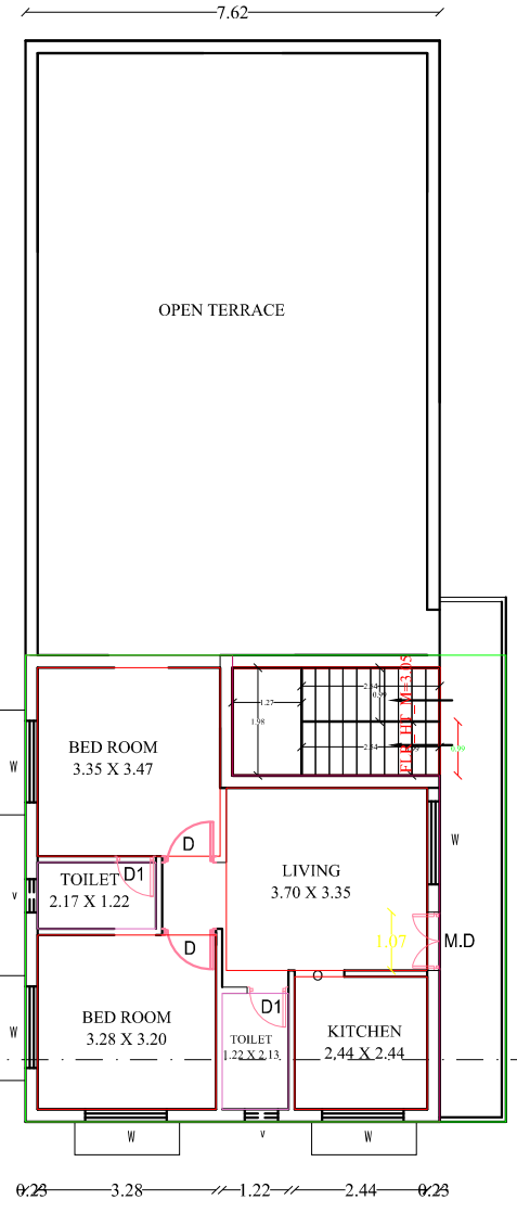
PRO. SECOND FLOOR PLAN
