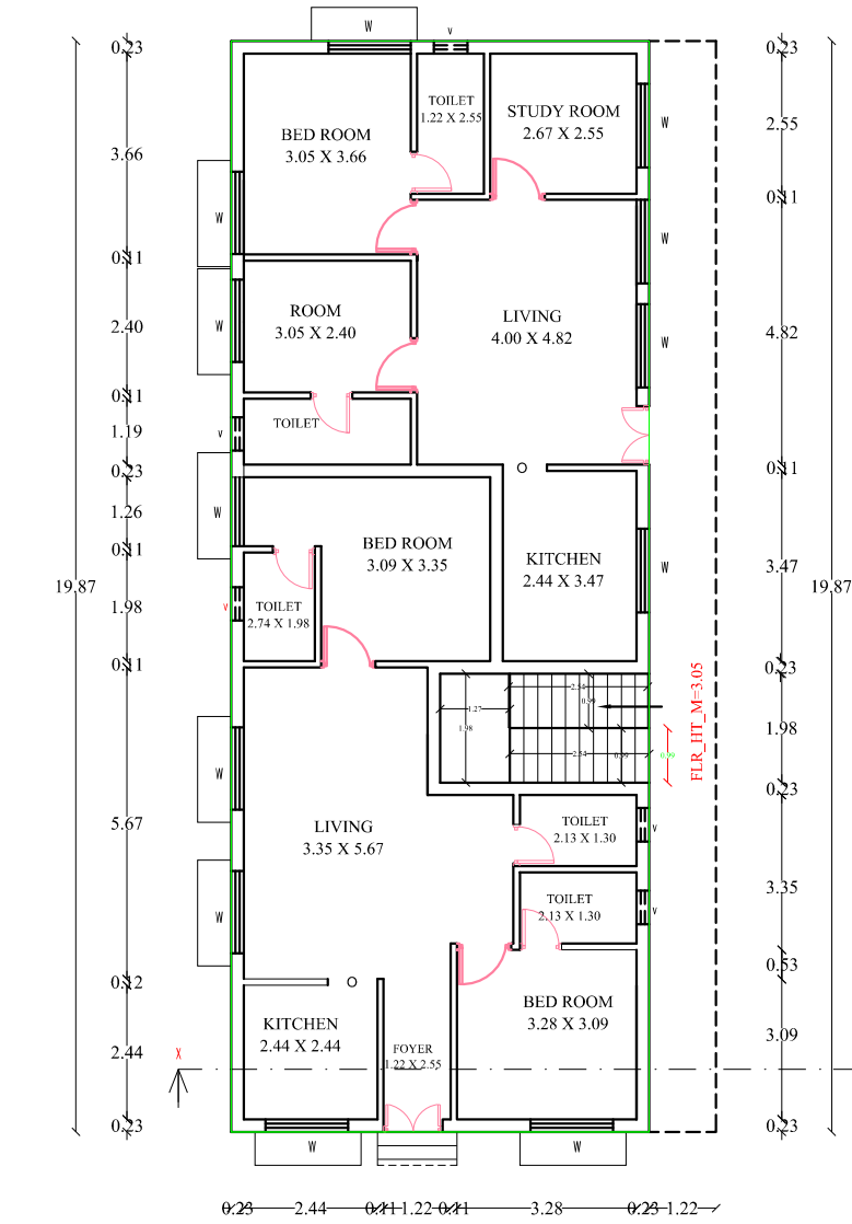
EXIST. GROUND FLOOR PLAN
