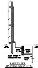
RAIN WATER HARVESTING SYSTEM
