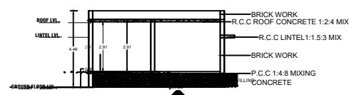
SECTION "A-B"
