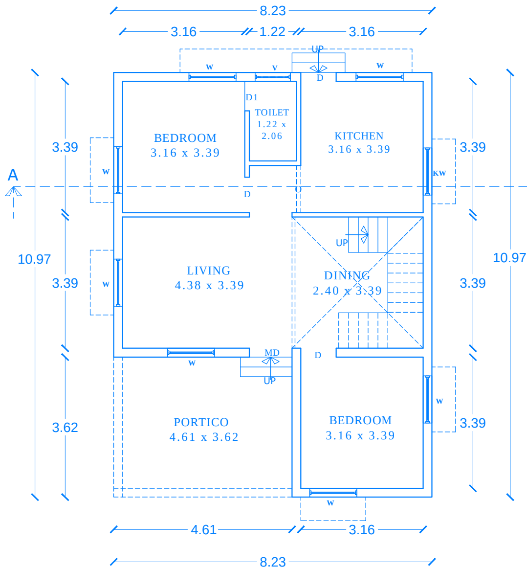
FLOOR PLAN
