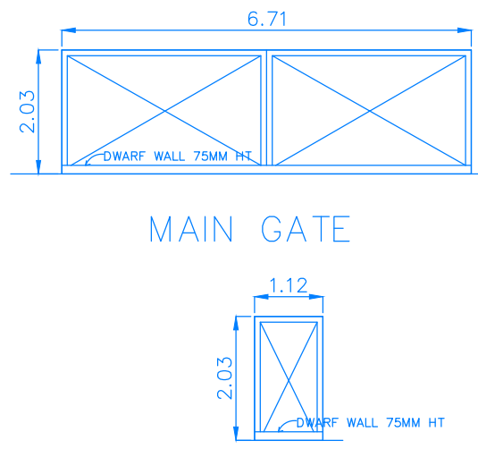
WICKET GATE
