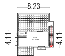
PRO FIRST FLOOR PLAN
