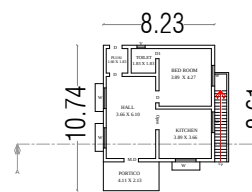
PRO GROUND FLOOR PLAN
