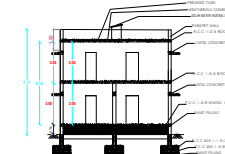
SECTION ON-'AA'
