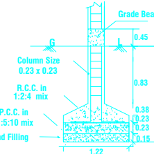
COLUMN DETAILS NOT TO SCALE
