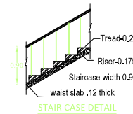
STAIR CASE DETAIL
