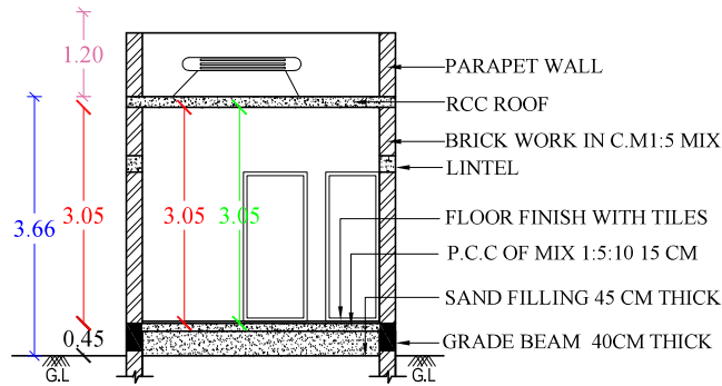
SECTION-AA1
