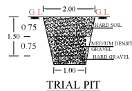
TRIAL PIT
