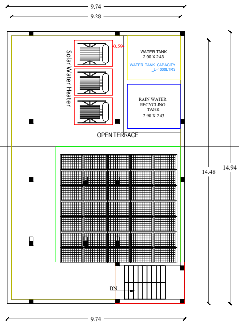
PRO.TERRACE FLOOR PLAN
