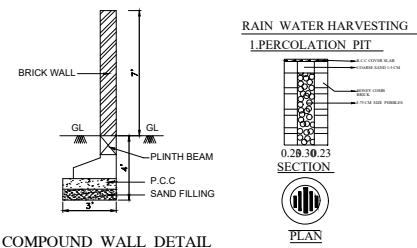
COMPOUND WALL DETAIL
