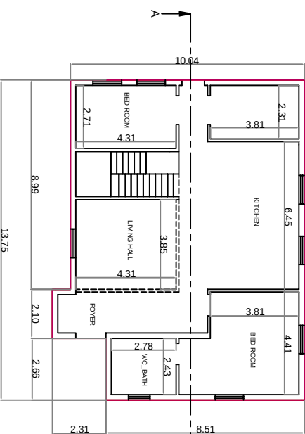
PROPOSED G . F. PLAN
