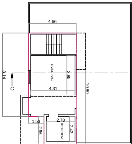
PROPOSED F . F. PLAN
