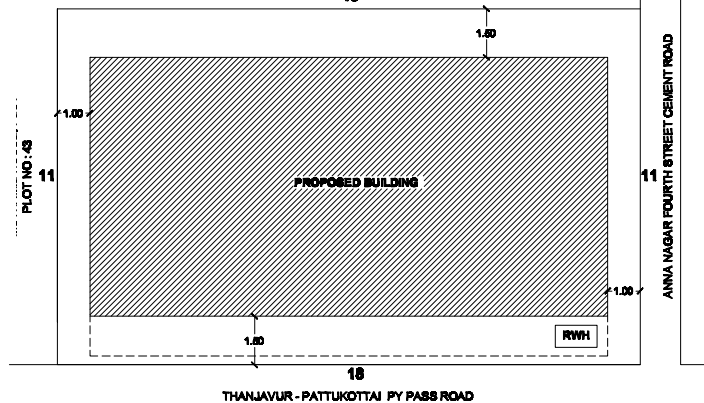
SITE PLAN
