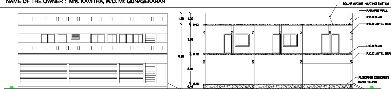
FRONT ELEVATION
