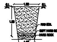
TRAIL PIT DETAIL
