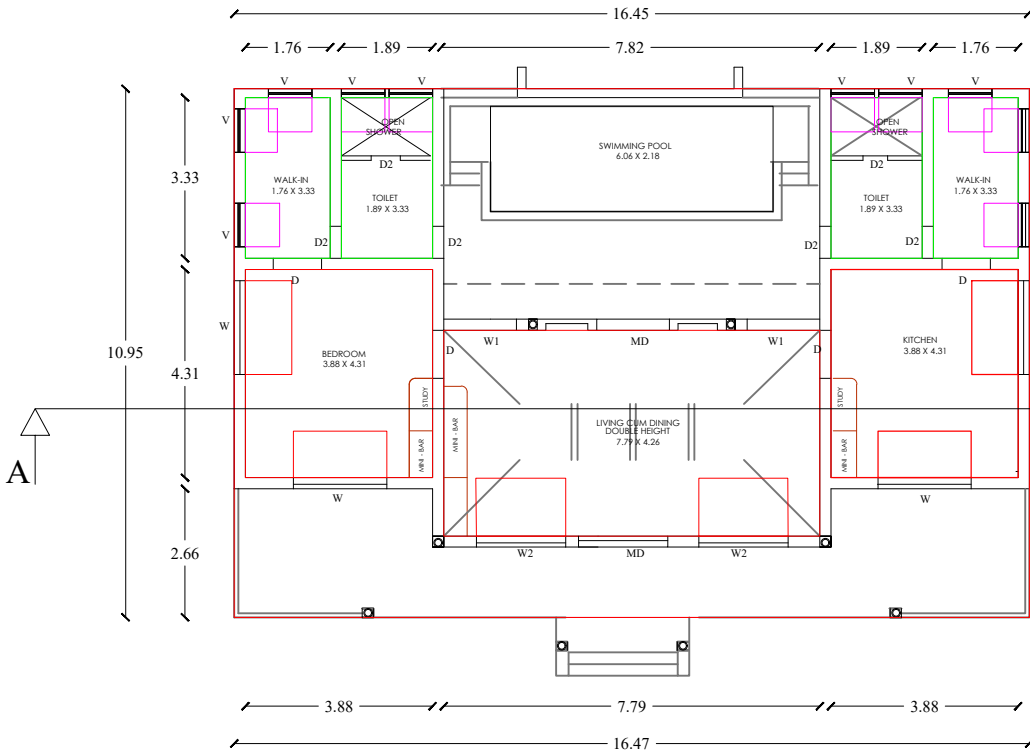
D FLOOR PLAN
